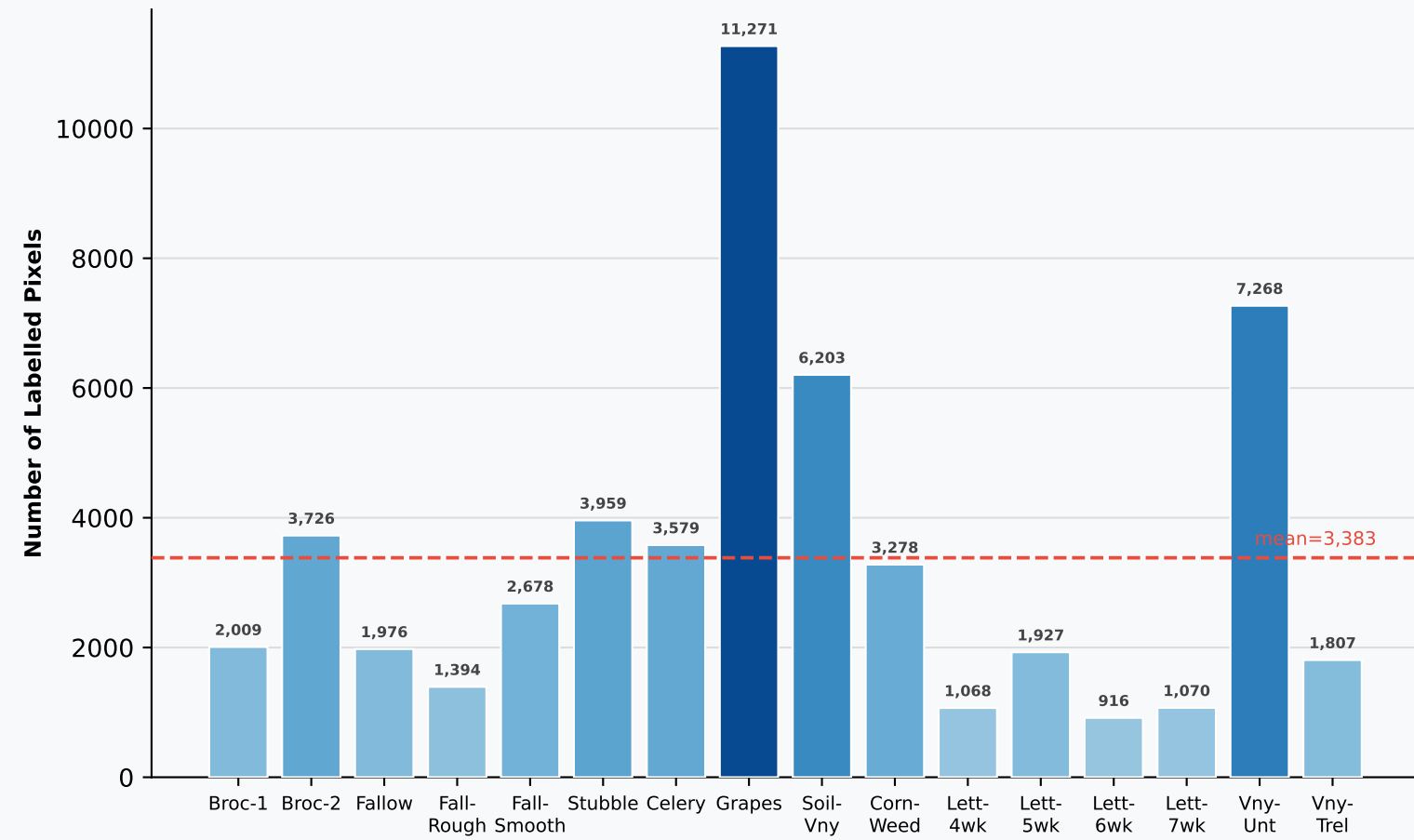
Salinas — Class Distribution
